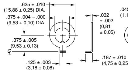
Non-Turn Washer
