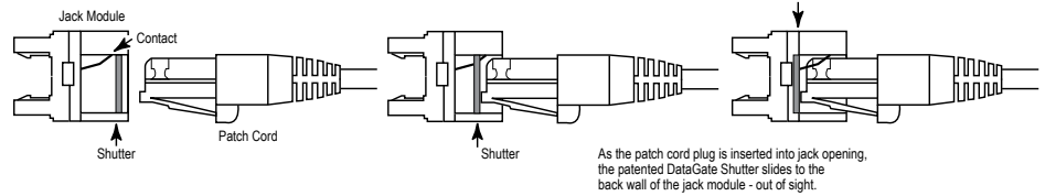
DataGate Shutter Operation
