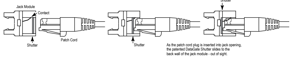
DataGate Shutter Operation
